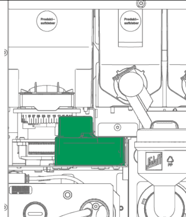
New grinder cover made from PA6
